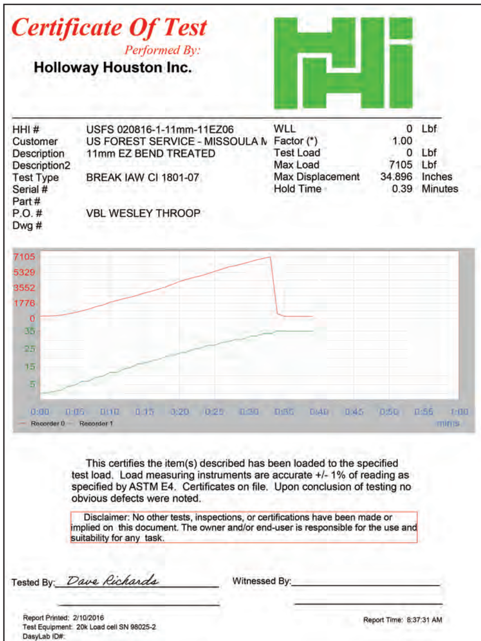
Figure 5—A certificate of test for a treated 11-millimeter EZ Bend rope sample. The red line and y-axis values indicate pound-force (lbf) applied to the rope. The green line and y-axis values indicate the amount of stretch or displacement of the rope in inches.
